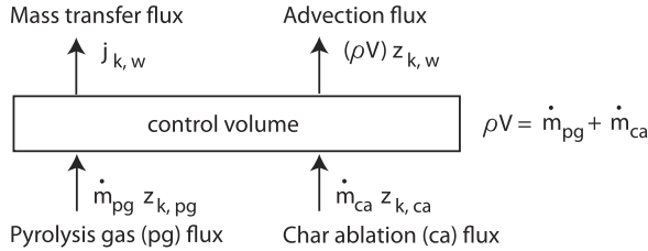
Fig. 3. Element mass-fraction conservation at the wall.
